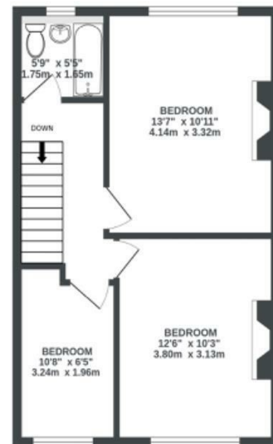
1ST FLOOR 423 sq.ft. (39.3 sq.m.) approx.
